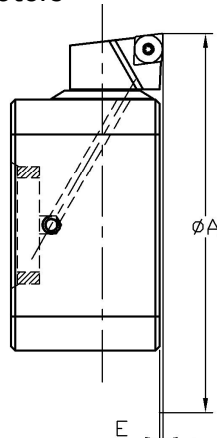
FIGURE 2 RHOMBOIDAL INDEXABLE
