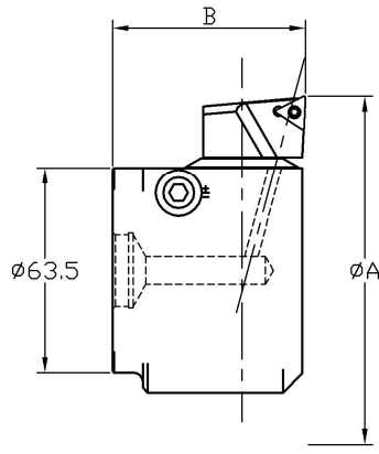
FIGURE 1 TRIANGULAR INDEXABLE
