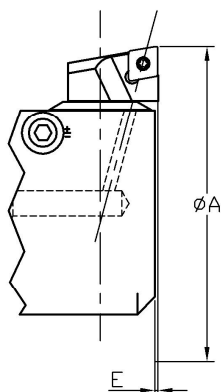
FIGURE 2 RHOMBOIDAL INDEXABLE
